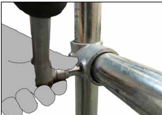
13. Ensure to fittings are torqued to 39Nm, that the pallet gate operates smoothly and is balanced.
