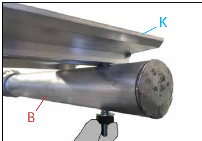
12. Add 1no. part (K) toe-board to part (B) uprights. Thread M10 bolt through hole in upright and add nut and washer. Tighten to 15Nm.
