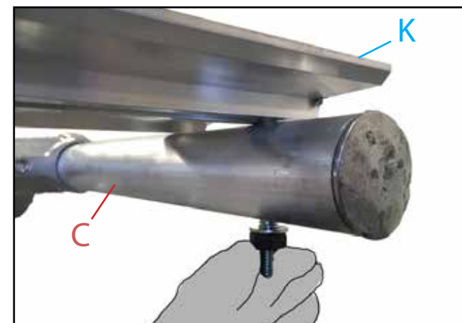
11. Add 1no. part (K) toe-board to part (C) uprights. Thread M10 bolt through hole in upright and add nut and washer. Tighten to 15Nm.
